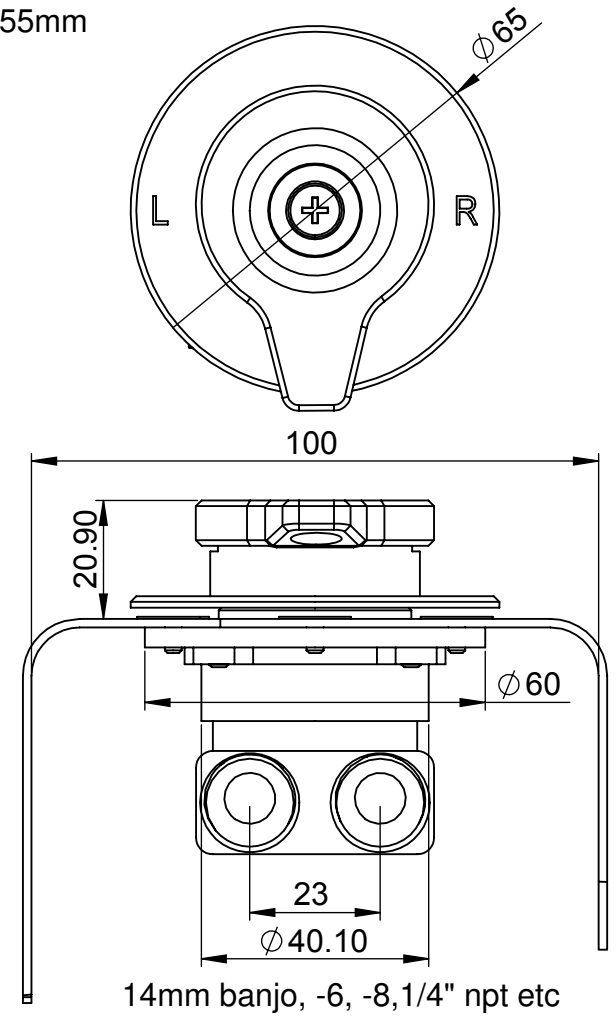
V7 - 17MM PORTS MASS 144g
